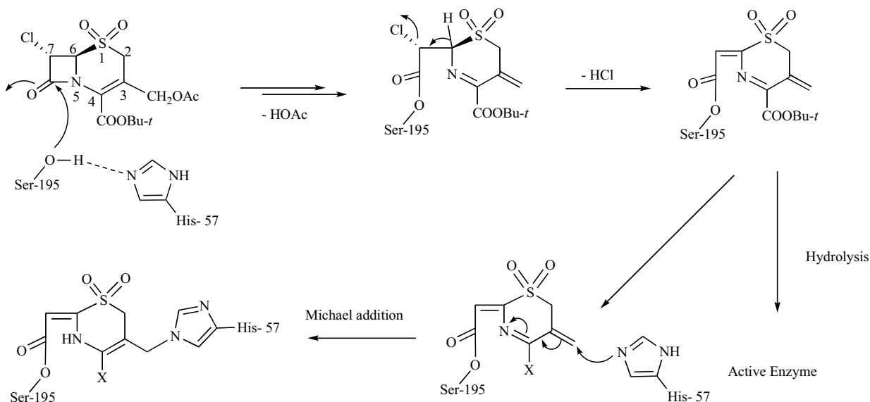
Fig. (17). The chemical mechanism for PPE inhibition [90, 96].
