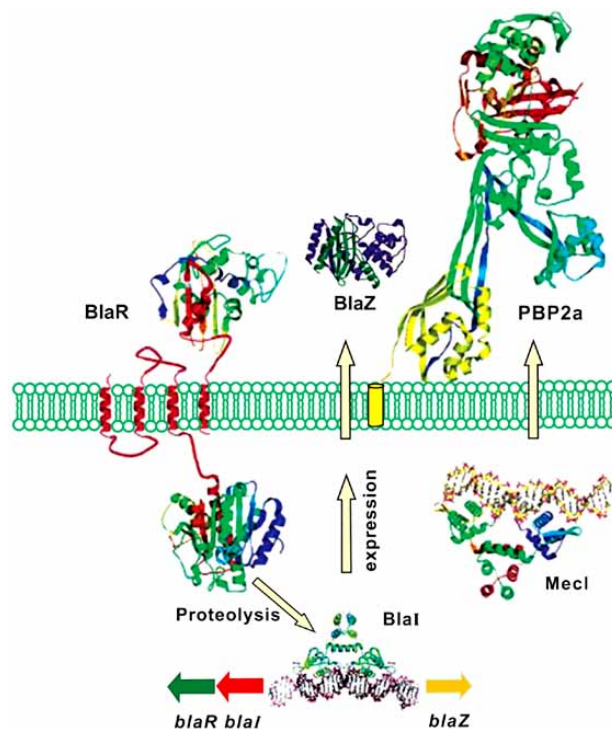
Fig. (3). Scheme of beta-lactam induced expression of \beta -lactamase and penicillin-binding protein 2a (PBP2a) in antibiotics resistant bacteria [15] (Copyright ACS).
