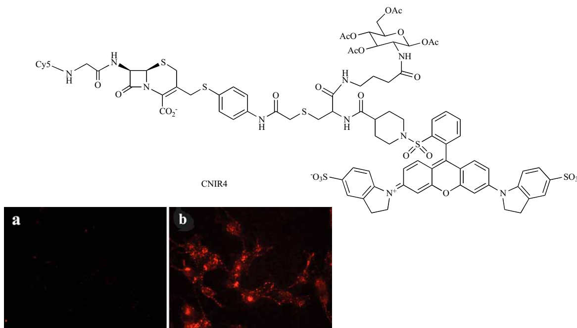
Fig. (8). Structure of CNIR4 and fluorescent images of wild-type (a) and Bla stably transfected (b) C6 Glioma cells staining with CNIR4 [61].
