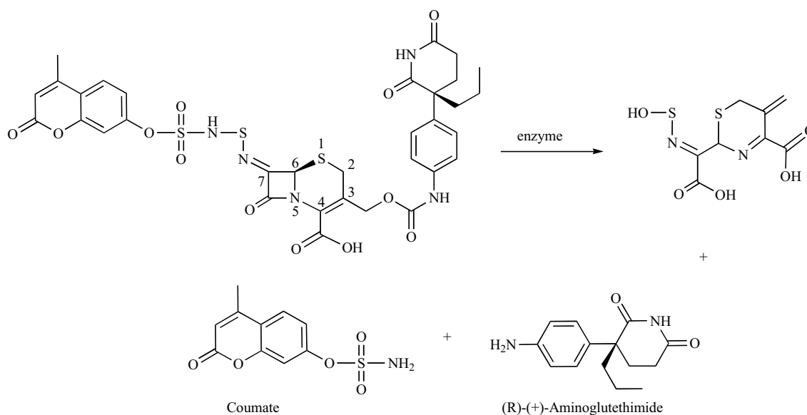
Fig. (13). Structure of dual release cephalosporin prodrug based on S-aminosulfenimine[78].
