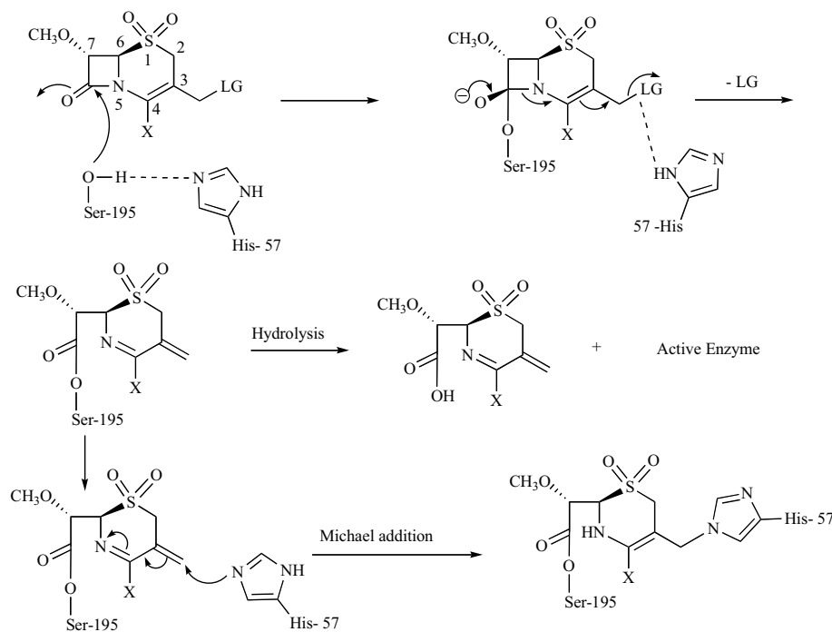
Fig. (15). Proposed chemical mechanism for the inhibition of HLE by the cephalosporin derivative [89].
