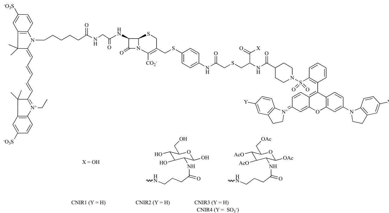
Fig. (7). Structures of CNIR1, CNIR2, CNIR3 and CNIR4 [61].
