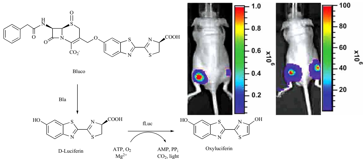
Fig. (9). Structure of Bluco and in vivo bioluminescent imaging Bla activity in living mice. COS7 cells ( 1 \times 10^6 ) were cotransfected with Bla and fLuc and injected into left rear thigh of a nude mouse, and the same number of cells transfected with fLuc only were injected at the right rear thigh [62].
