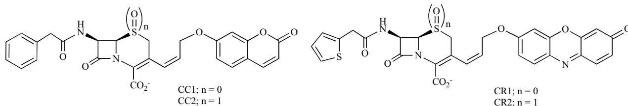
Fig. (5). Structures of CC1, CC2, CR1 and CR2 [59].
