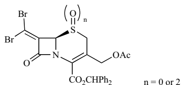
Fig. (16). Structure of 7-alkylidenecephalosporin derivatives [90].
