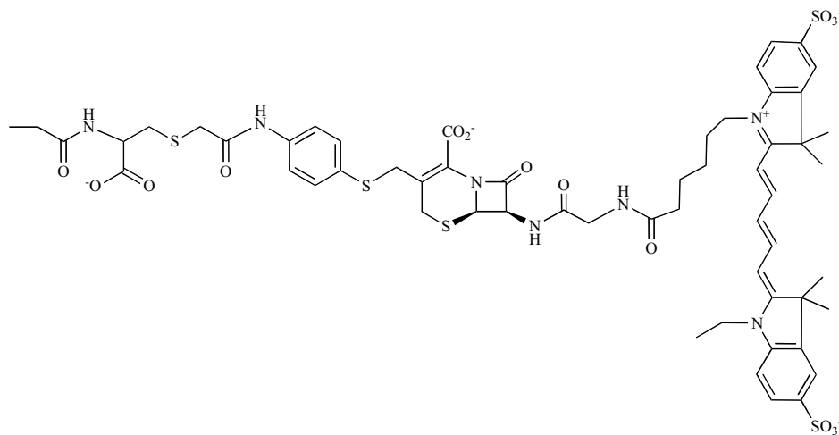
Fig. (10). Structure of QDot-based nanosensor for detecting Bla [64].
