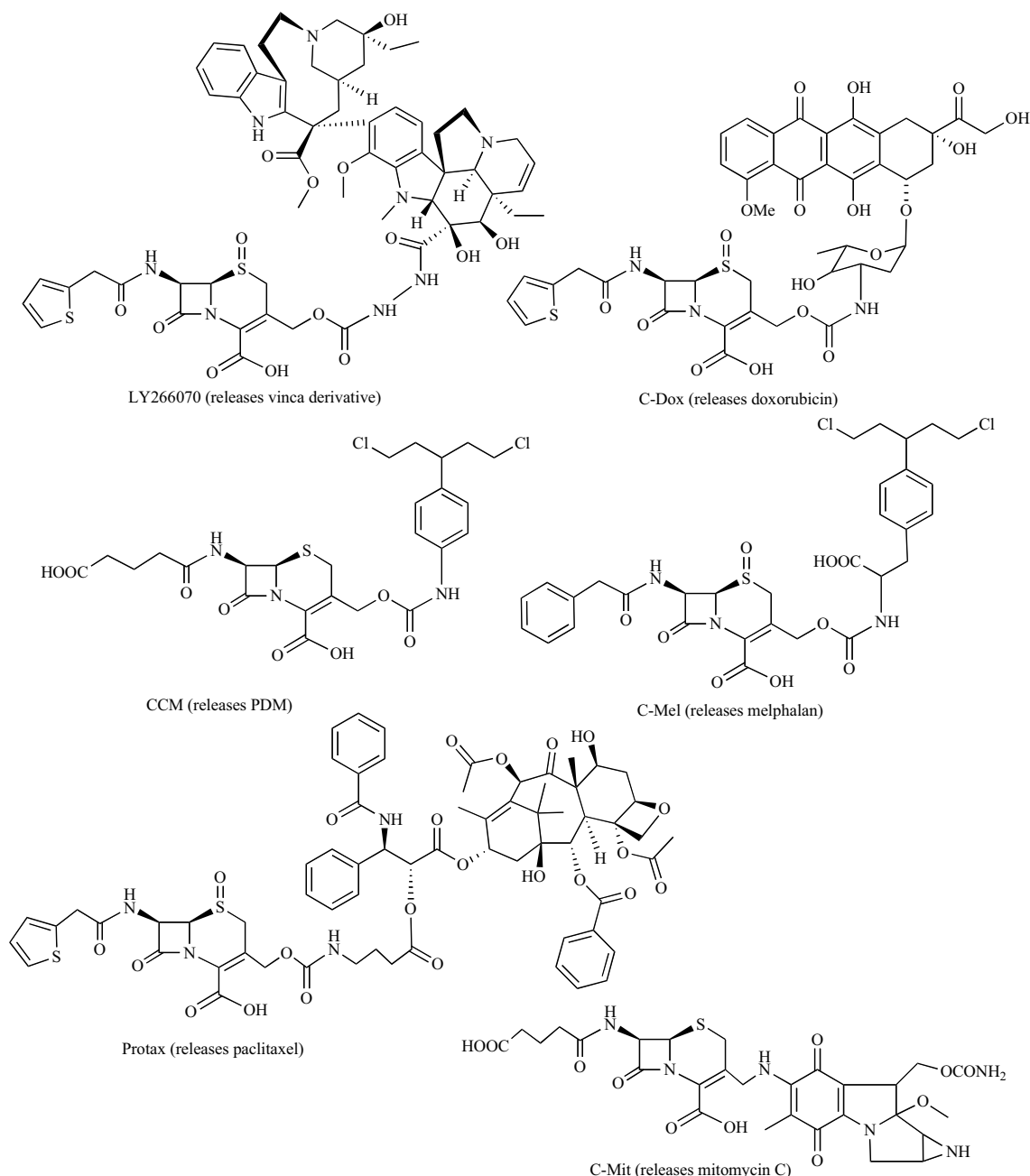
Fig. (11). Structures of some \beta -lactamase targeted prodrugs.
