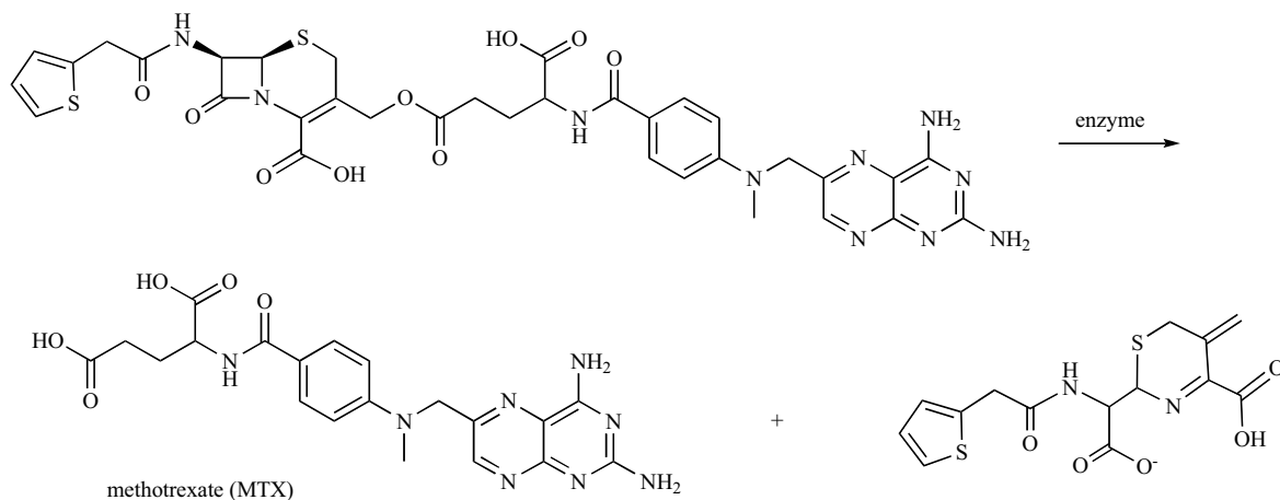
Fig. (12). Structure and reaction scheme of cephalosporin methotrexate prodrug [69].
