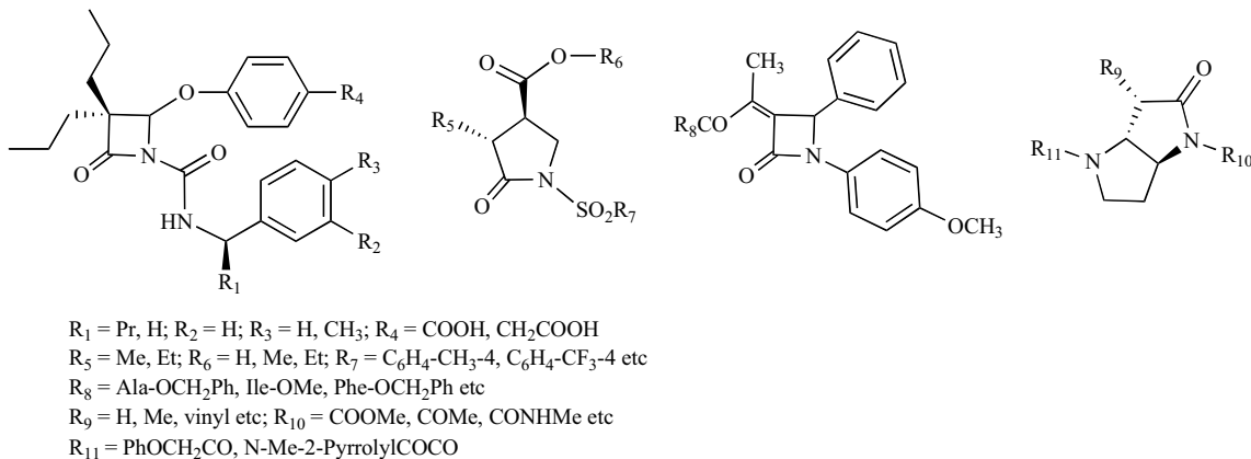
Fig. (19). Structures of monocyclic \beta -lactam and other cyclic lactam systems [100-107].
