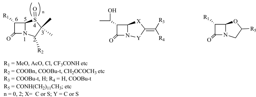
Fig. (18). Structures of penicillins derivatives [89, 92].
