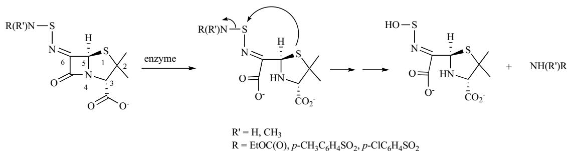
Fig. (14). Structure and reaction scheme of S-aminosulfenimine based penicillin prodrug.
