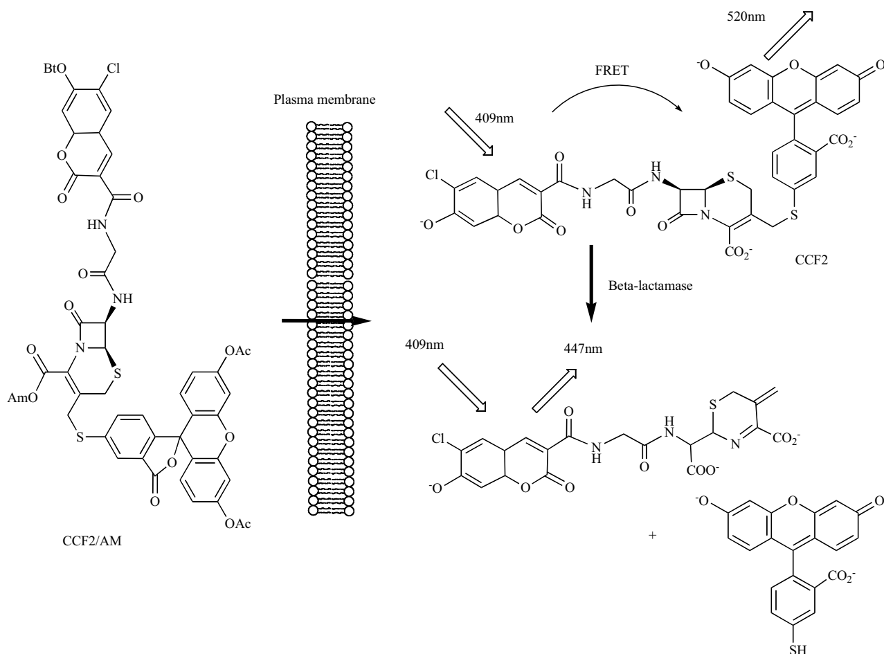
Fig. (4). Mechanism of action in the FRET in CCF2/AM [41].
