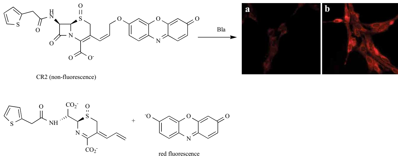
Fig. (6). Fluorescence images of wild-type (a) and Bla-stably transfected (b) C6 glioma cells incubated with CR2/AM [59].
