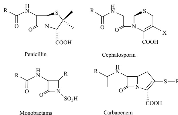
Fig. (1). Structure of the \beta -lactam antibiotics.
